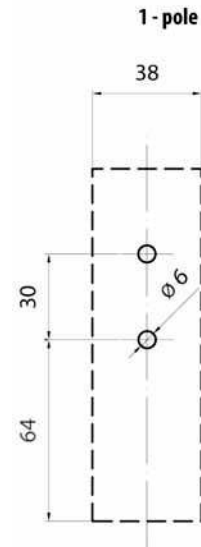
Clearance and drilling plans for BHF000-1A/T (1 pole), for BHF000-3A/T (3 poles) multiply the width by 3
