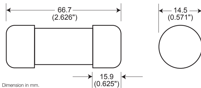
Fig. 1: 20-30 Amp Range
